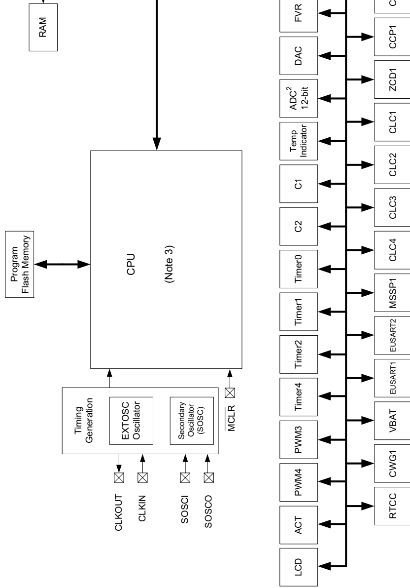
FIGURE 1-1: PIC16(L)F19155/56/75/76/85/86 BLOCK DIAGRAM
