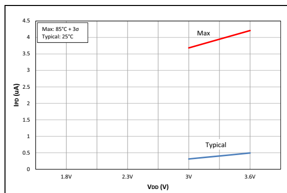
FIGURE 40-27: IPD, Low-Power Brown-Out Reset (LPBOR), PIC16LF19155/56/75/76/85/86 Only.
