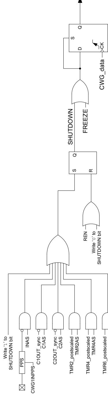
FIGURE 31-12: CWG SHUTDOWN BLOCK DIAGRAM
