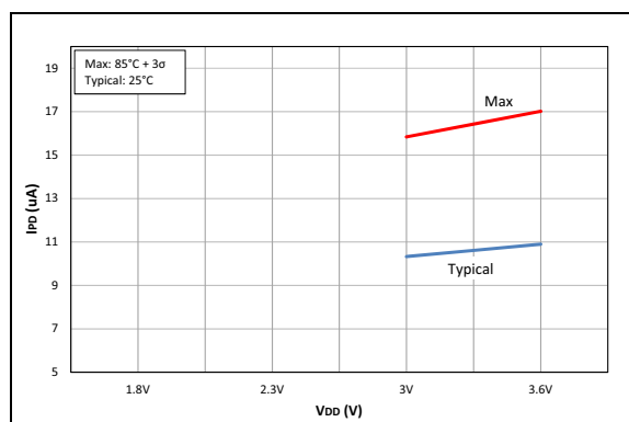
FIGURE 40-28: IPD, Brown-Out Reset (BOR), PIC16LF19155/56/75/76/85/86 Only.
