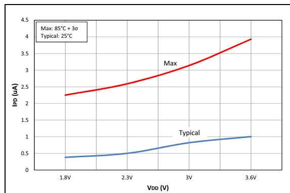
FIGURE 40-29: IPD, Secondary Oscillator (SOSC), PIC16LF19155/56/75/76/85/86 Only.
