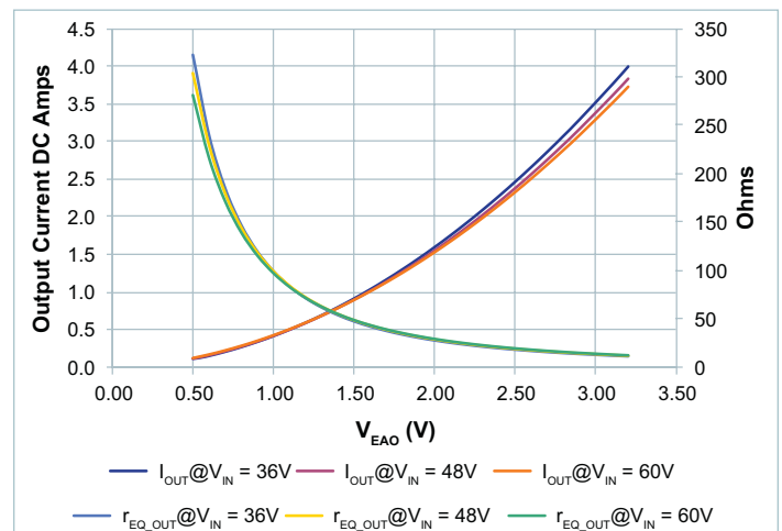
Figure 98 — r_{EQ\_OUT} vs. output current vs. V_{EAO} , V_{OUT} = 36V ; 36 - 60V_{IN}
