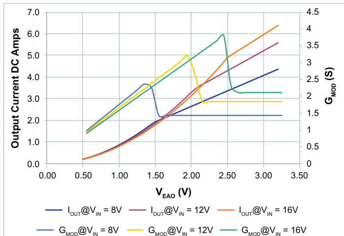
Figure 75 — G_{MOD} vs output current vs. V_{EAO} , V_{OUT} = 18\text{V} ; 8 - 16V_{IN}
