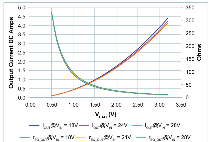
Figure 97 — r_{EQ\_OUT} vs. output current vs. V_{EAO} , V_{OUT} = 36V ; 18 - 28V_{IN}
