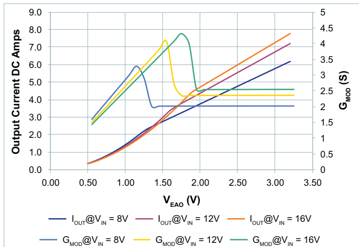
Figure 63 — G_{MOD} vs output current vs. V_{EAO} , V_{OUT} = 10V ; 8 - 16V_{IN}
