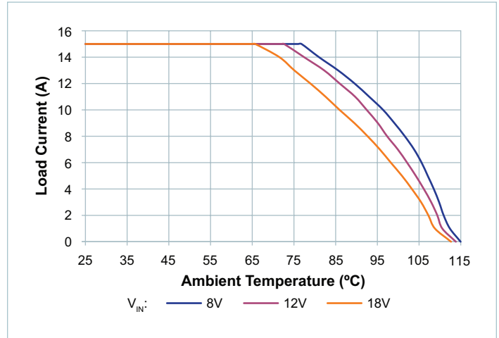
Figure 14 — PI3424 – load current vs. ambient temperature, OLFM
