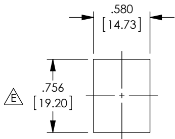
RECOMMENDED PANEL OPENING
