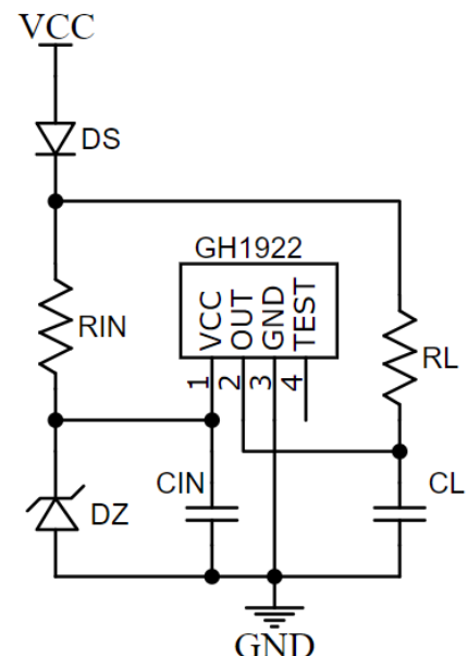
B. Application under unstable power supply
