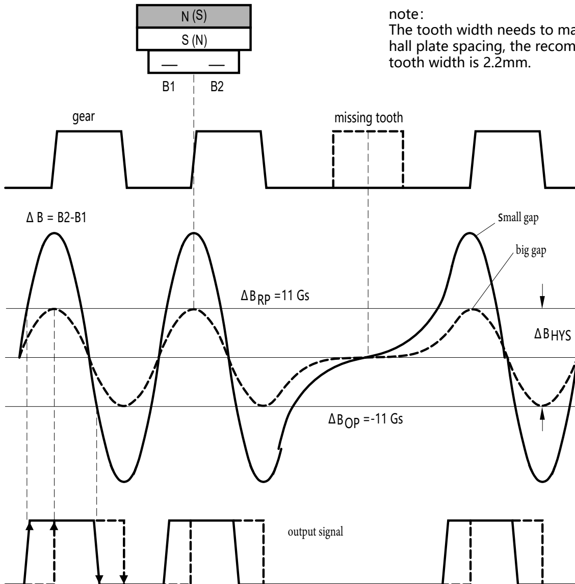
Fig.3 The basic working principle of GH1922 when used as a gear sensor
