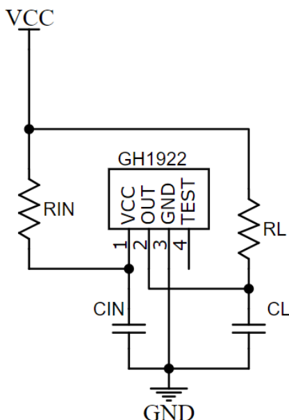
A. Application under stable power supply
