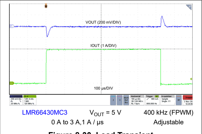
Figure 8-30. Load Transient
