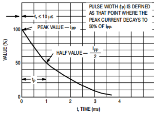
Figure 5. Pulse Waveform
