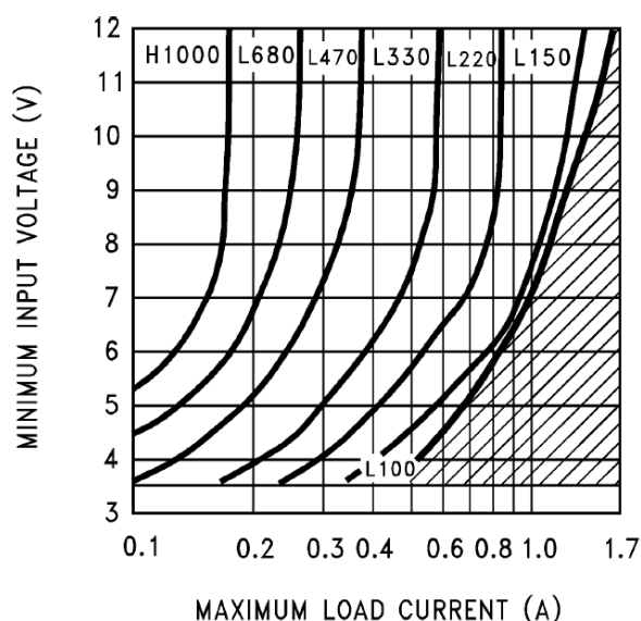
FIGURE 8. LM2577S/T_ADJ-15
