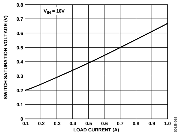
Figure 15. Switch Saturation Voltage vs. Load Current
