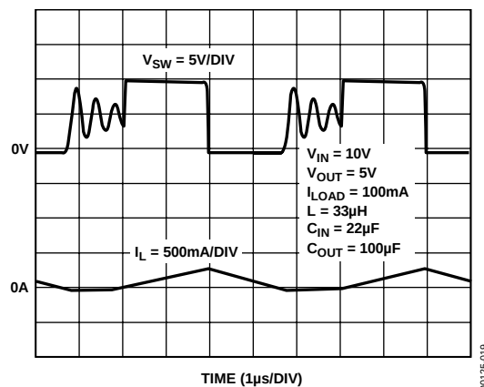
Figure 19. Discontinuous Conduction Mode Waveforms
