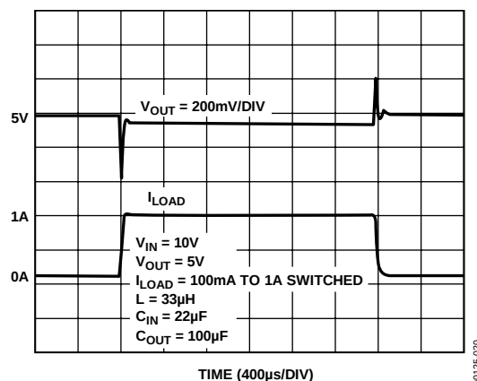
Figure 20. Transient Response
