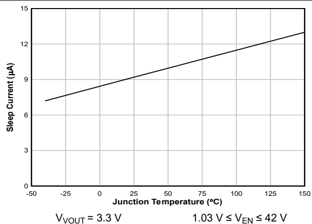
Figure 7-4. Sleep1 Current vs Temperature
