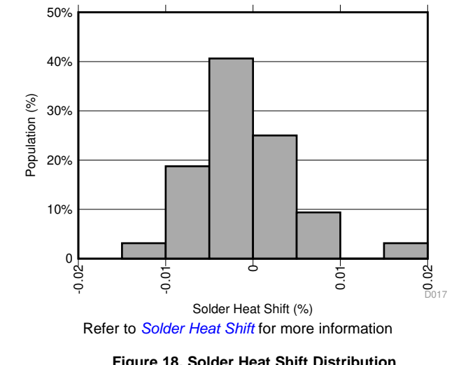
Figure 18. Solder Heat Shift Distribution
