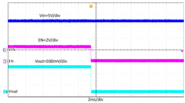
Figure 8-19. Shutdown Through EN, I OUT = 4 A
