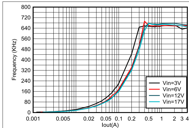
Figure 8-2. TPS564252 Frequency vs Loading
