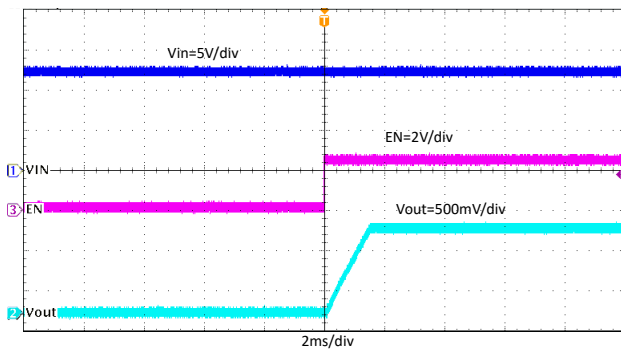
Figure 8-18. Start-Up Through EN, I OUT = 4 A
