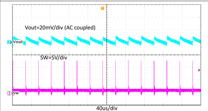
Figure 8-13. TPS564255 Output Voltage Ripple with 0.01-A Loading
