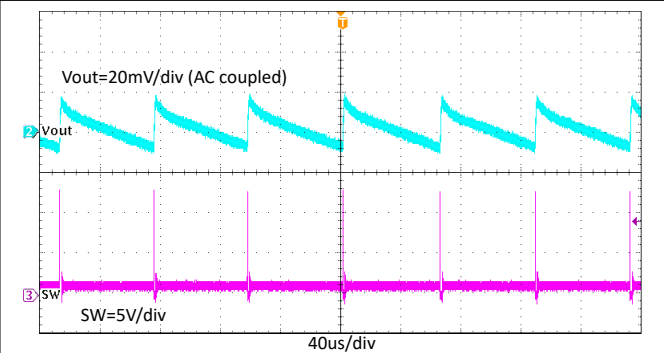
Figure 8-11. TPS564252 Output Voltage Ripple with 0.01-A Loading
