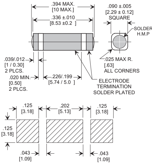
SUGGESTED MOUNTING PATTERN
