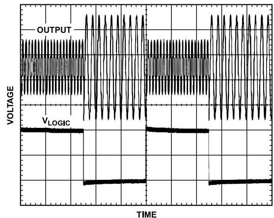
Figure 101. Multiplexed Output
