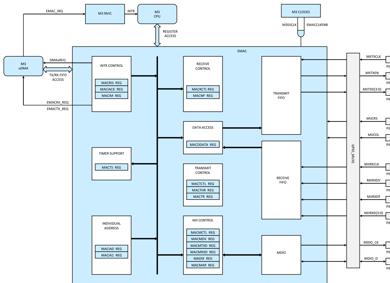
Figure 7-35. EMAC
