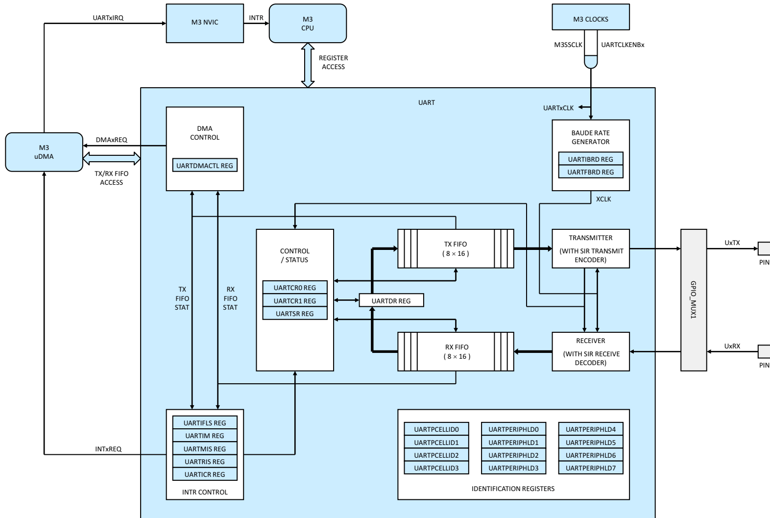
Figure 5-32. UART
