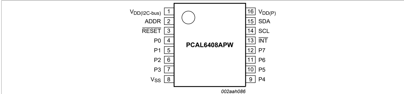
Figure 2. Pin configuration for TSSOP16
