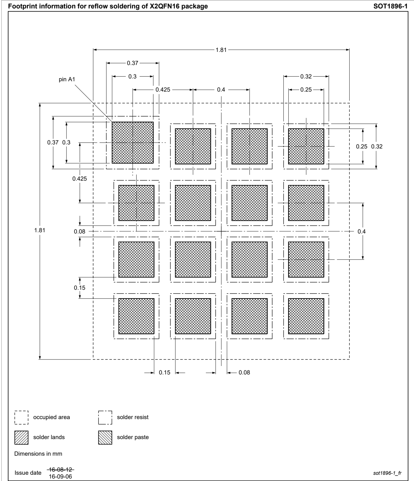
Figure 45. PCB footprint for SOT1896-1 (X2QFN16); reflow soldering
