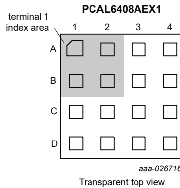
Figure 6. Pin configuration for 1.6 mm × 1.6 mm X2QFN16 EX1 land grid array
