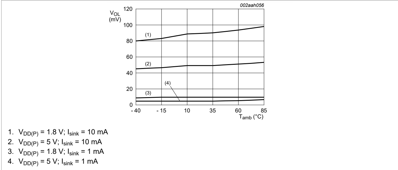
Figure 30. LOW-level output voltage versus temperature
