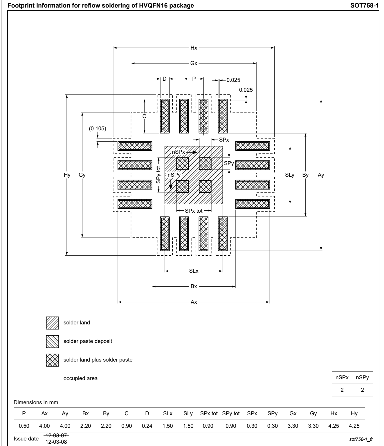
Figure 42. PCB footprint for SOT758-1 (HVQFN16); reflow soldering
