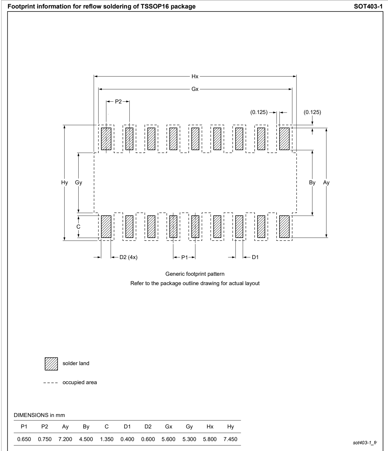
Figure 43. PCB footprint for SOT403-1 (TSSOP16); reflow soldering
