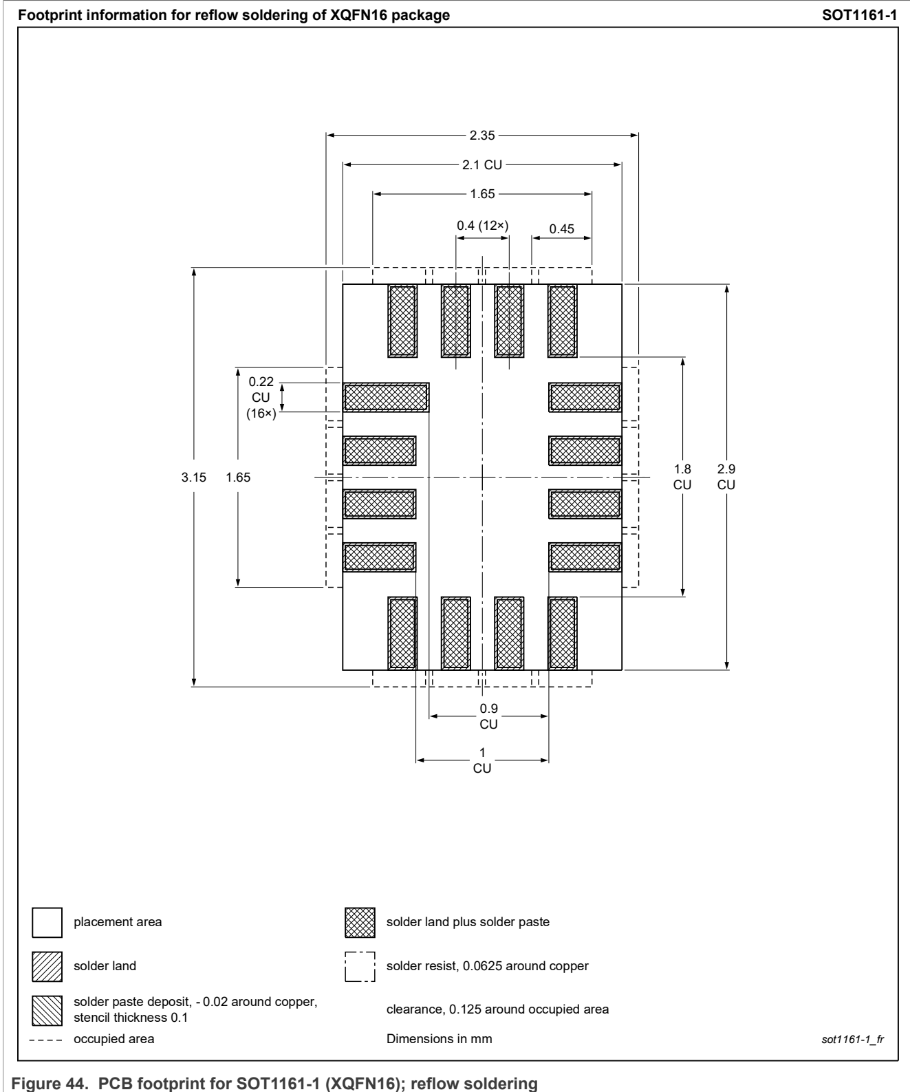
Figure 44. PCB footprint for SOT1161-1 (XQFN16); reflow soldering
