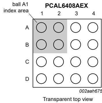
Figure 5. Pin configuration for 1.6 mm × 1.6 mm XFBGA16
