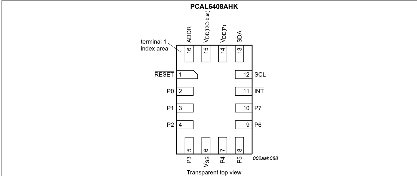
Figure 4. Pin configuration for XQFN16
