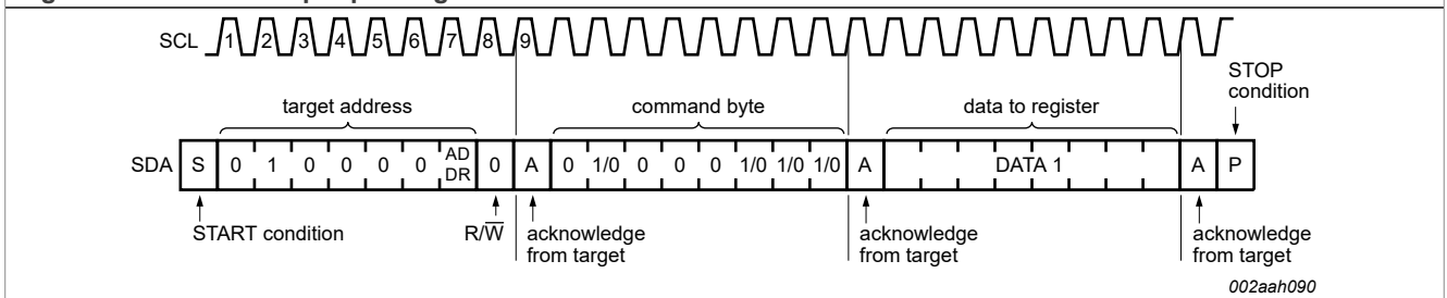
Figure 12. Write to Configuration or Polarity inversion registers
