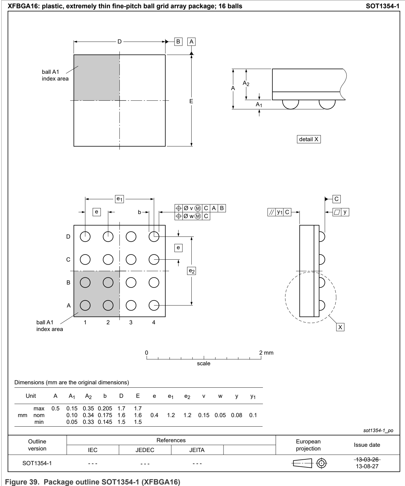
Figure 39. Package outline SOT1354-1 (XFBGA16)
