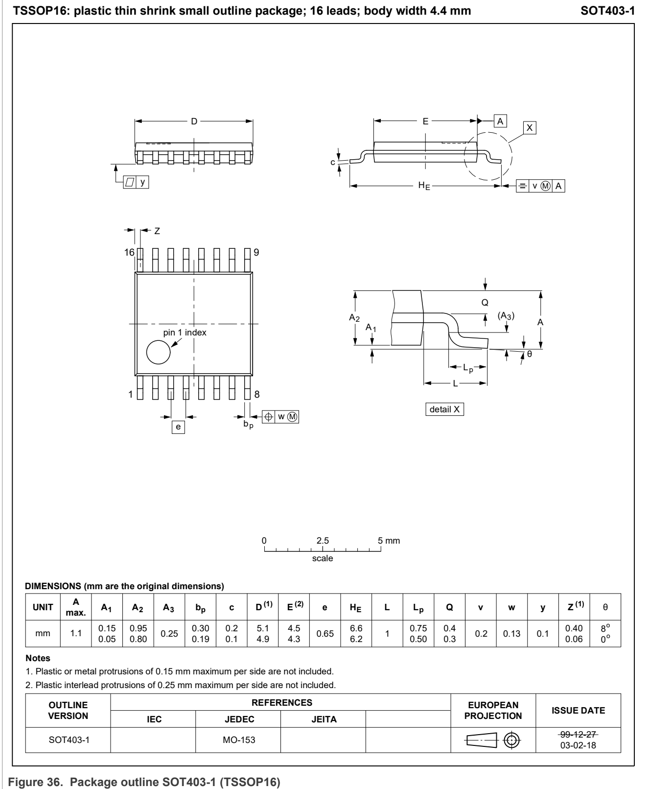
Figure 36. Package outline SOT403-1 (TSSOP16)
