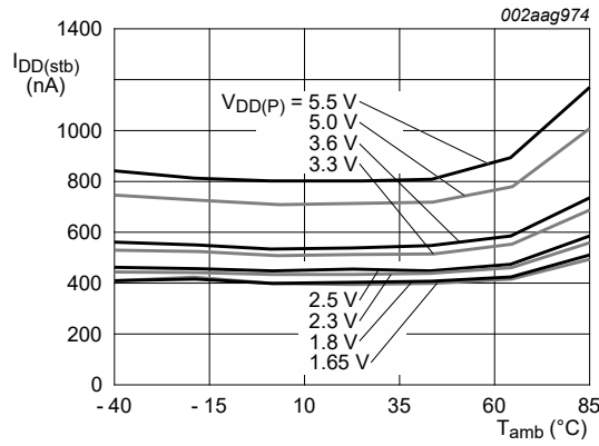
Figure 25. Standby supply current versus ambient temperature
