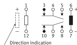
Schematic ( BOTTOM VIEW ) ( Reset ) ( Operation function LT )
