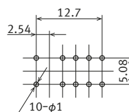
Recommended PC board pattern ( BOTTOM VIEW )
