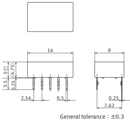
PC board terminal ( self-clinching terminal )
