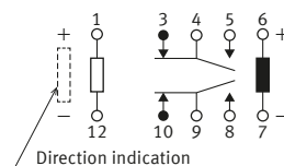
Schematic ( BOTTOM VIEW ) ( Reset ) ( Operation function LT )
