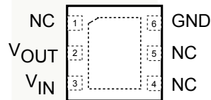
Figure 2. 6-Lead, 3x3mm MLP(Top View)
