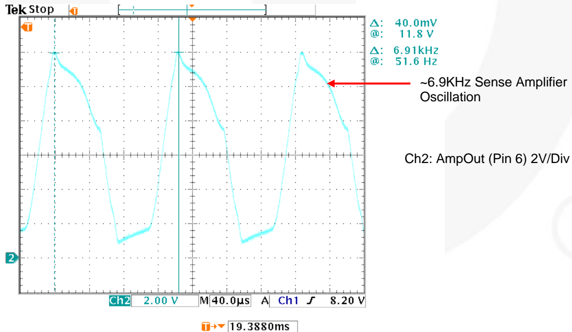
Figure 9. Typical Waveform for Grounded Neutral Detection
