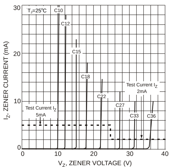
Figure 4 Typical Zener Breakdown Characteristics
