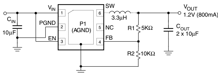
Figure 1. Typical Application
