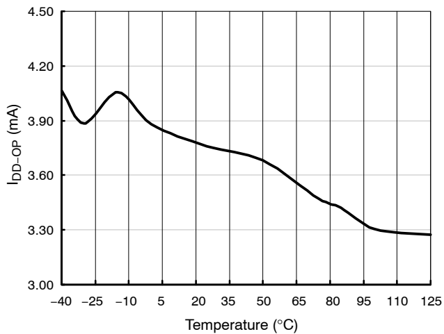
Figure 8. Operating Current
