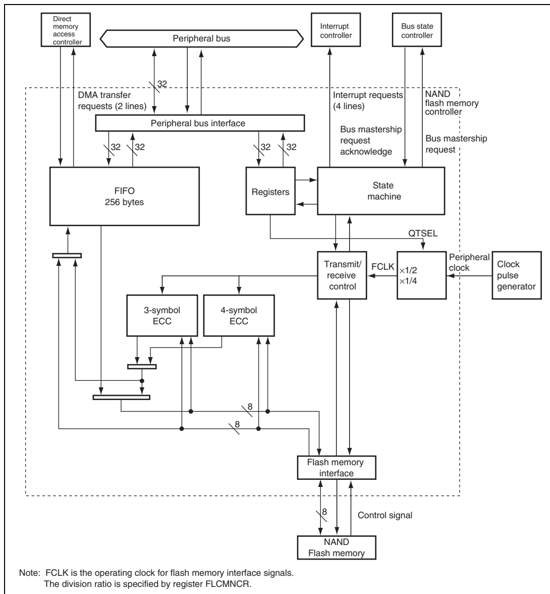
Figure 25.1 Block Diagram
