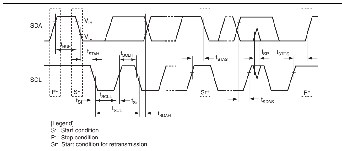
Figure 37.52 (1) Input/Output Timing
