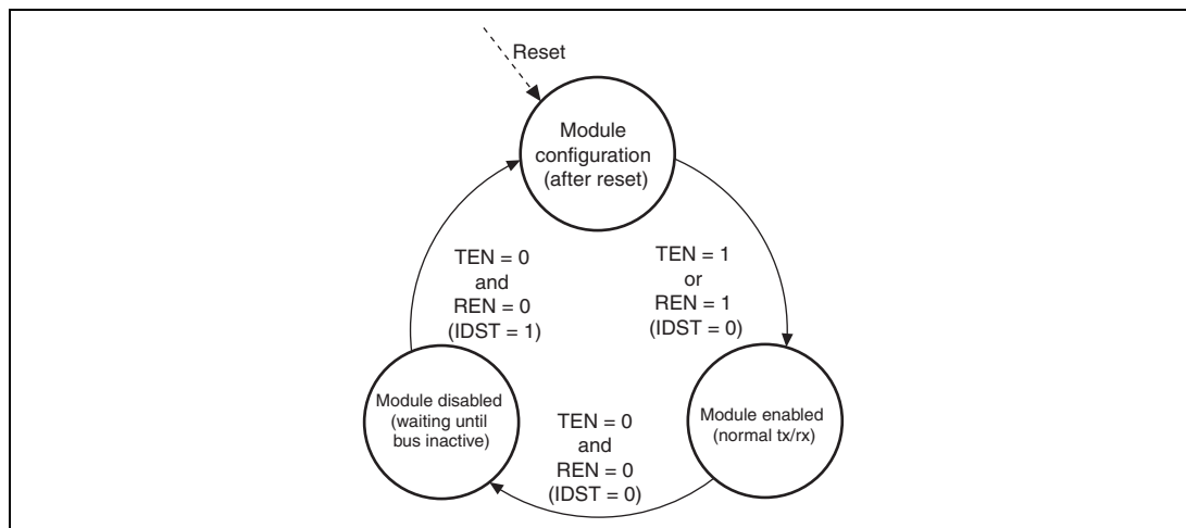
Figure 18.19 Operation Modes
