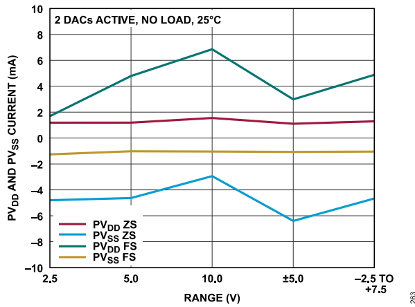
Figure 78. PV_{DD} and PV_{SS} Current vs. Range
