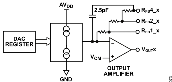
Figure 79. DAC Channel Architecture Block Diagram
