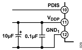
Figure 30. V_{DDP} Bias and Bypass Components
