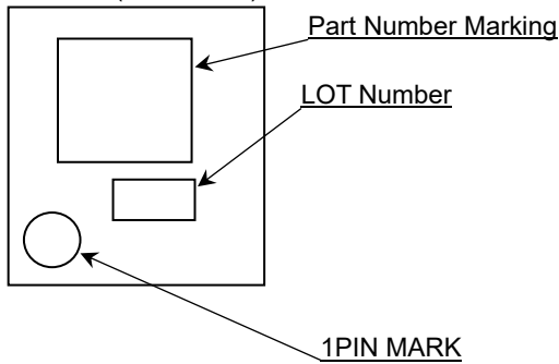
HSON8 (TOP VIEW)
