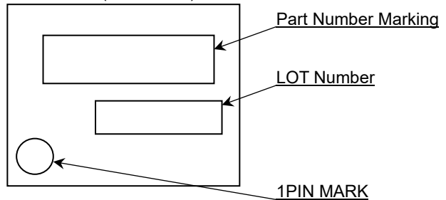
HTSOP-J8(TOP VIEW)
