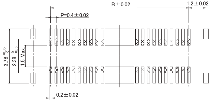
DF40HB (Retention Tab)
