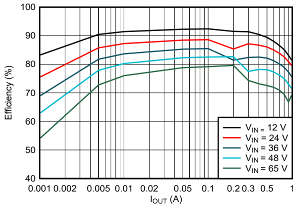
f_{SW} = 1.1\text{ MHz} V_{OUT} = 5\text{ V} LMR51610Y
