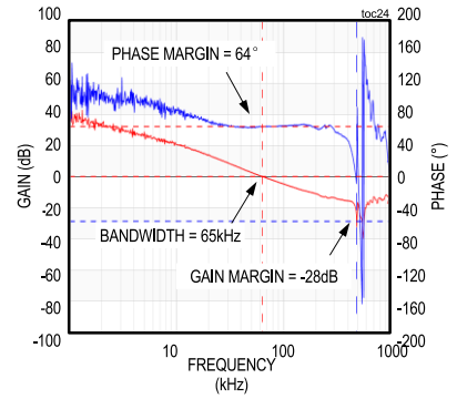
BODE PLOT ( V_{OUT} = 1.0V , I_{OUT} = 15A , f_{SW} = 500kHz )
