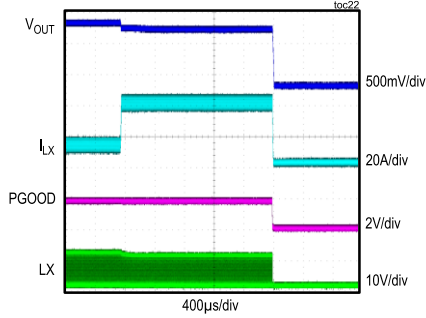
POSITIVE OVERCURRENT PROTECTION ( V_{OUT} = 1.0V , f_{SW} = 500kHz , POCP = 38A )
