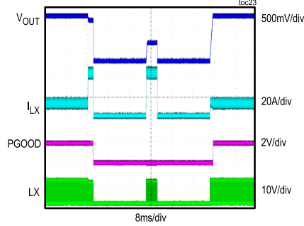
POCP HICCUP AND AUTORETRY ( V_{OUT} = 1.0V , f_{SW} = 500kHz , POCP = 38A )
