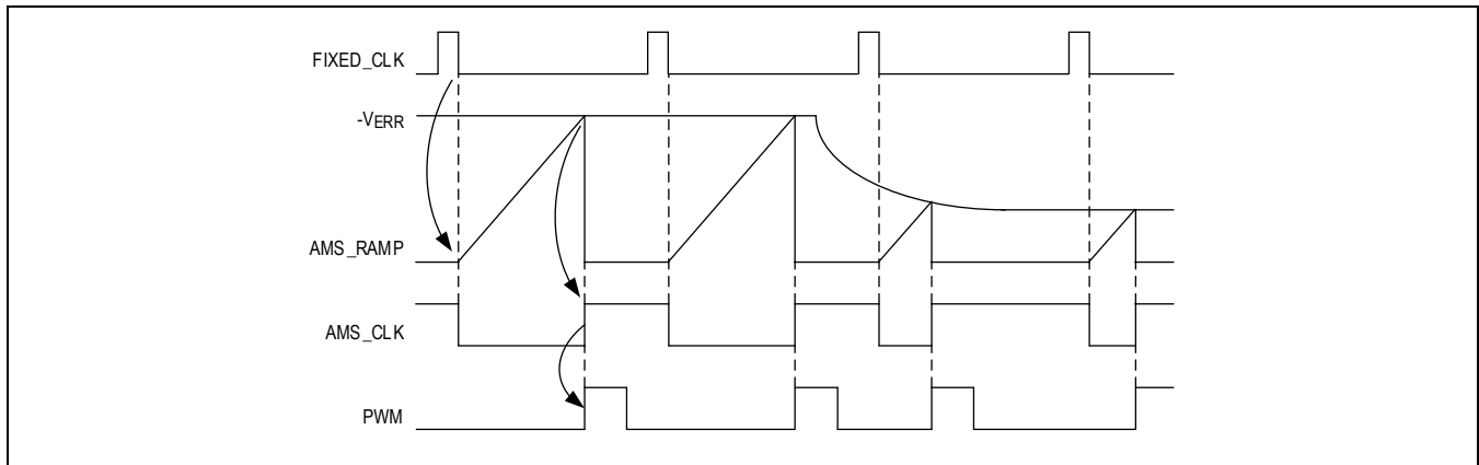
Figure 2. AMS Operation
