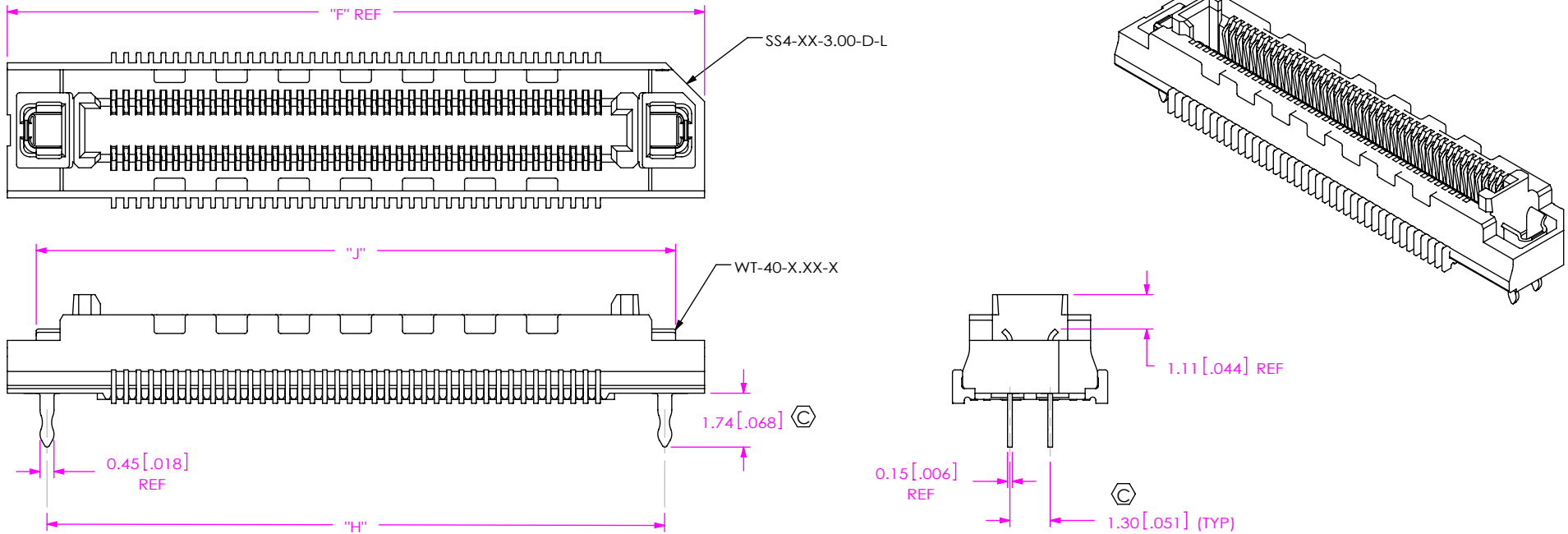
FIG 3 -L: LATCHING OPTION SS4-40-3.00-X-D-L SHOWN (DIFFERENT AS SHOWN, OTHERWISE SAME AS FIG 1)
