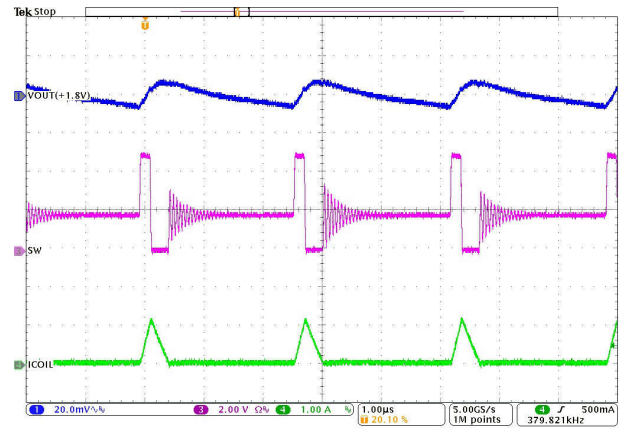
I_{OUT} = 100\text{ mA} PFM Figure 8-30. Output Voltage Ripple
