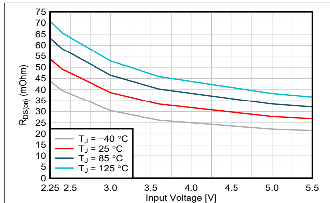
Figure 6-1. High-Side FET On-Resistance
