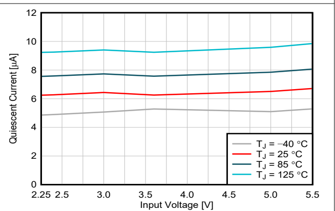
Figure 6-4. Quiescent Current
