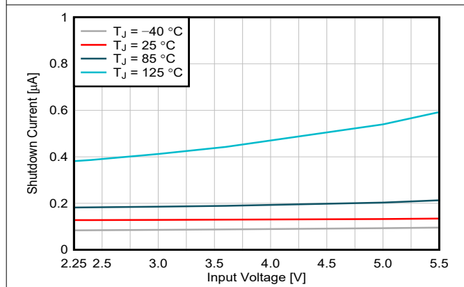
Figure 6-3. Shutdown Current
