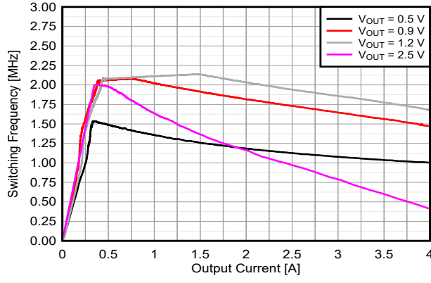
V_{IN} = 3.3\text{ V} PFM Figure 8-27. Switching Frequency versus Output Current
