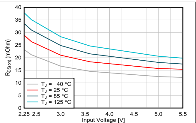
Figure 6-2. Low-Side FET On-Resistance
