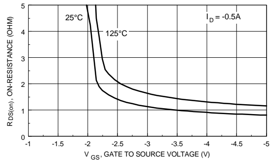
Figure 14. On Resistance Variation with Temperature.
