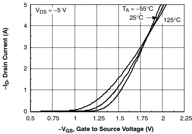
Figure 5. Transfer Characteristics
