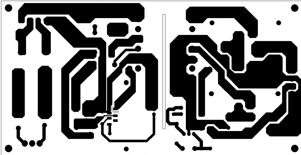
Figure 26. Layout Considerations for FSDM0465RS
