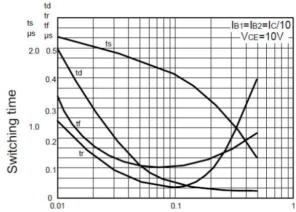
Switching Speeds
