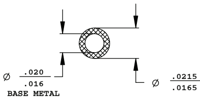
SECTION X-X
