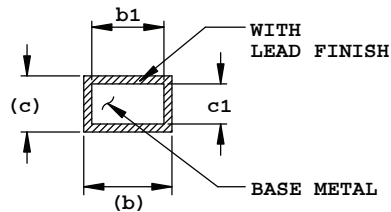
SECTION Z-Z
