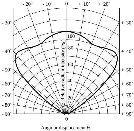
Fig.12 Radiation Diagram (GL513F)
