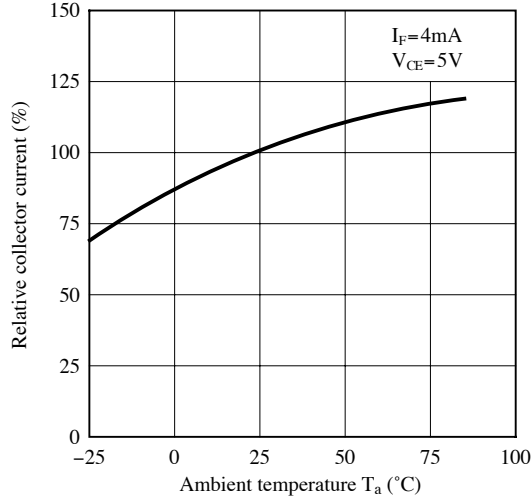
Fig.7 Relative Collector Current vs. Ambient Temperature
