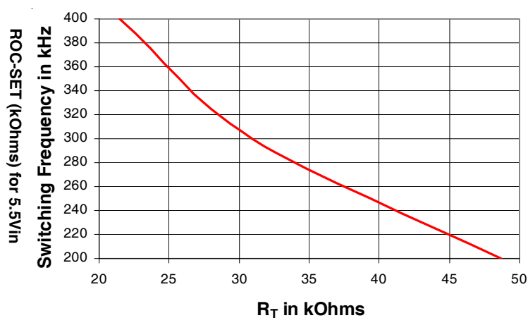
Fig. 9: Per Channel Switching Frequency vs R_T www.irf.com
