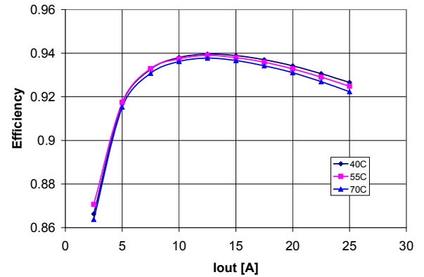
Fig. 4: Efficiency vs. load current and ambient temperature for converter mounted vertically with V_{in} = 48 V and air flowing from pin 4 to pin 1 at a rate of 200 LFM (1.0 m/s).
