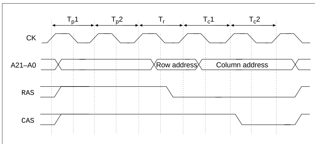
Figure 8.19 Precharge Timing (Long Pitch)
