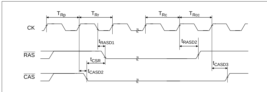
Figure 19.31 Self Refresh
