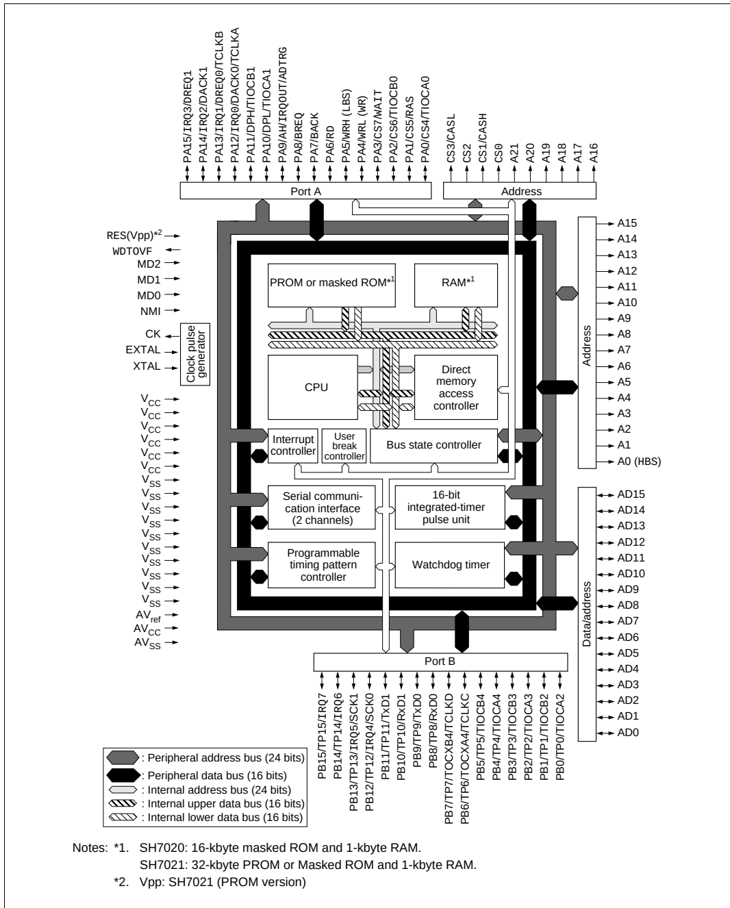
Figure 1.1 Block Diagram
