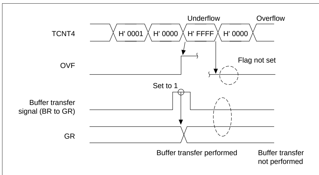
Figure 10.37 Undershoot Timing
