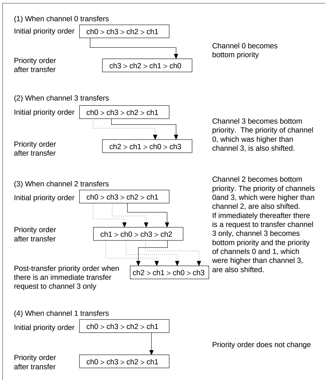
Figure 9.3 Round-Robin Mode
