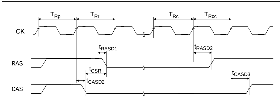
Figure 19.18 Self Refresh
