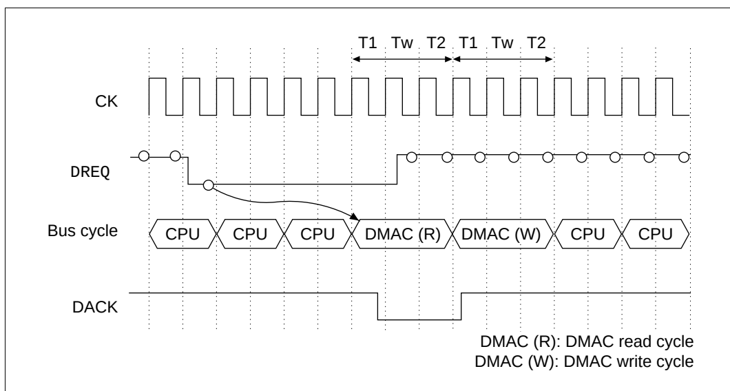
Figure 9.18 \overline{\text{DREQ}} Sampling Timing in Cycle Steal Mode (Output with \overline{\text{DREQ}} level detection and \overline{\text{DACK}} active low) (Dual address mode, bus cycle = 2 states + 1 wait state)
