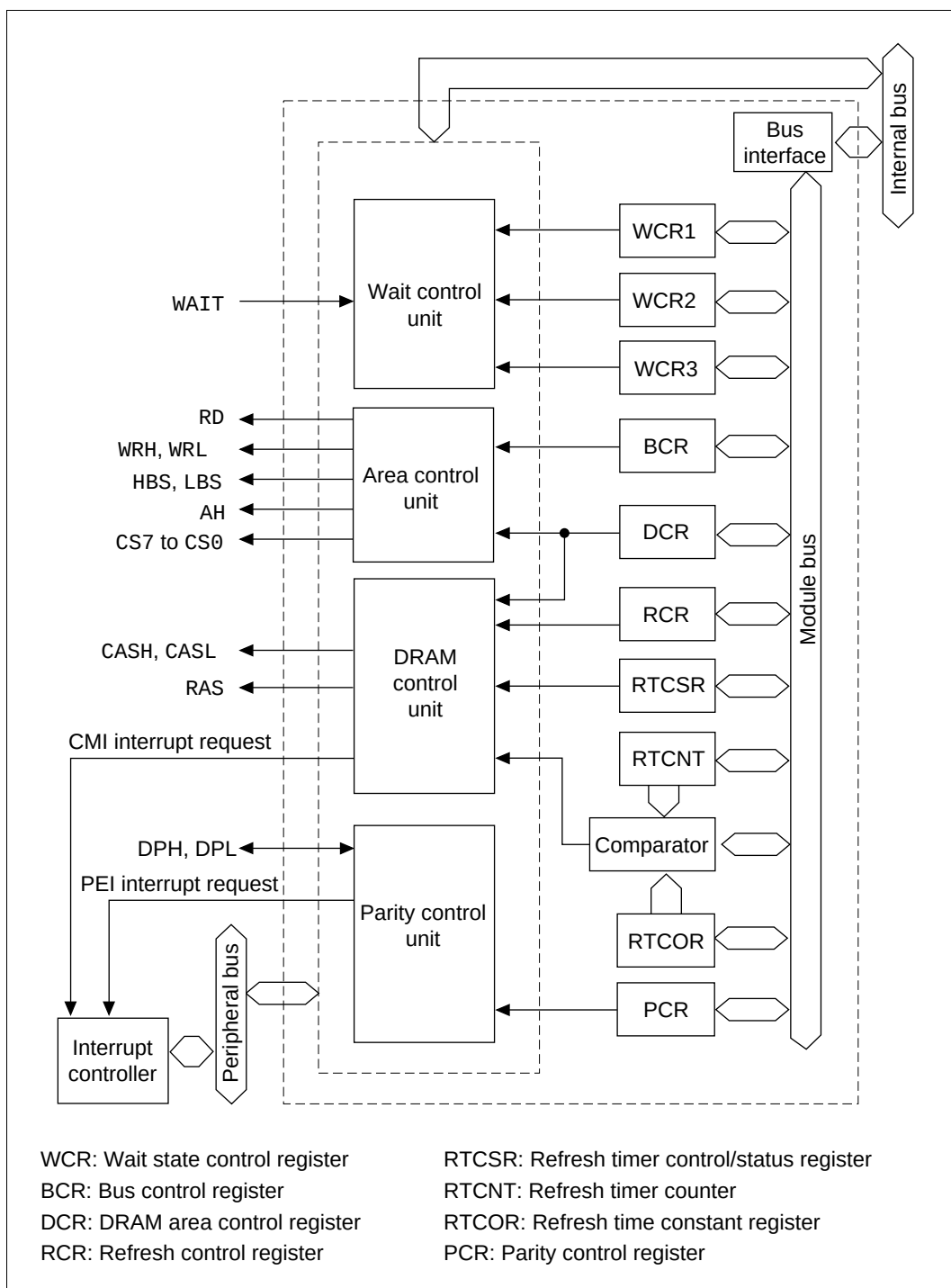
Figure 8.1 BSC Block Diagram
