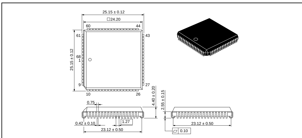
Figure E-4. Package Dimensions (CP-68)
