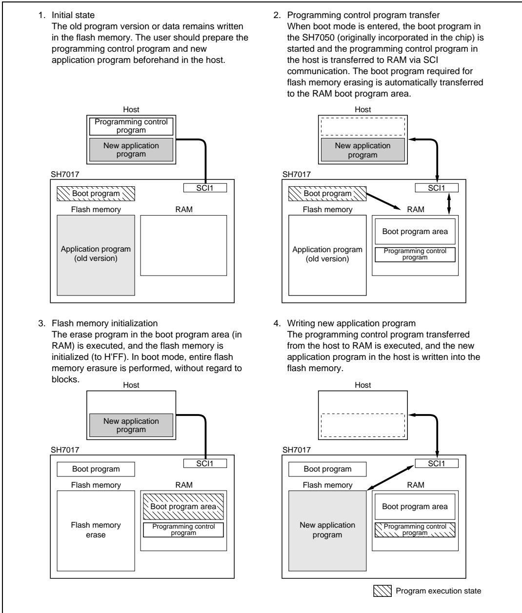
Figure 18.3 Boot Mode
