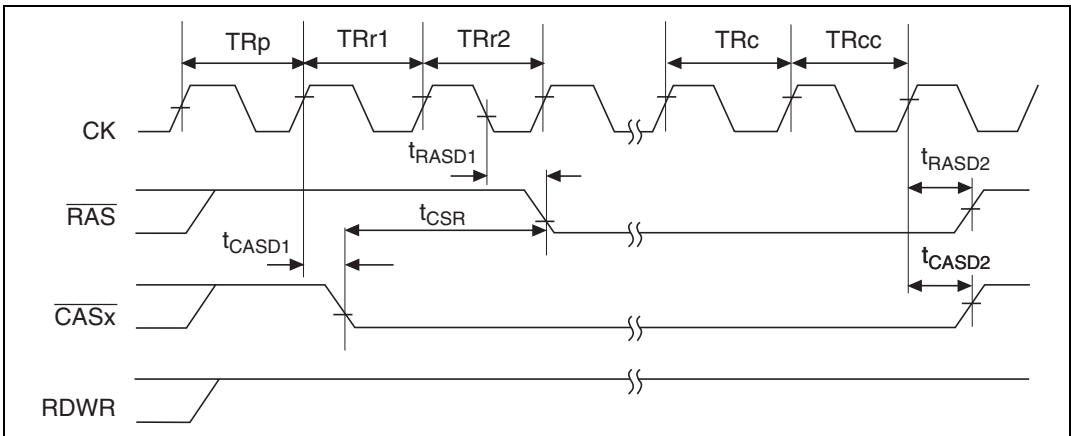
Figure 22.16 Self Refresh
