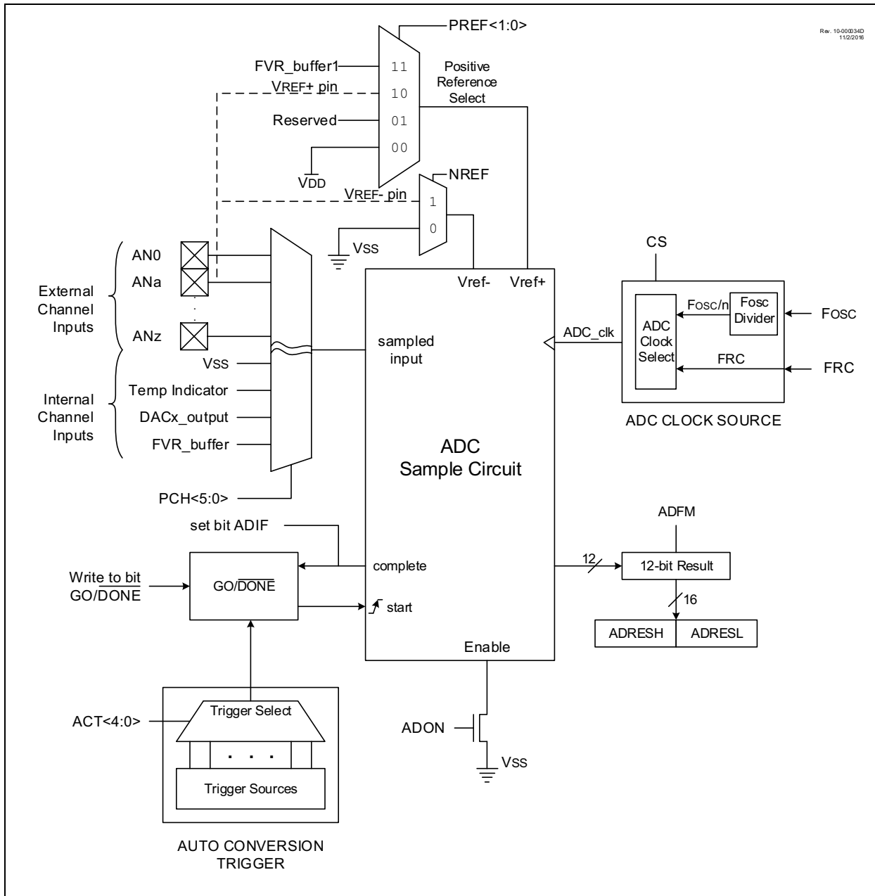
FIGURE 37-1: ADC 2 BLOCK DIAGRAM
