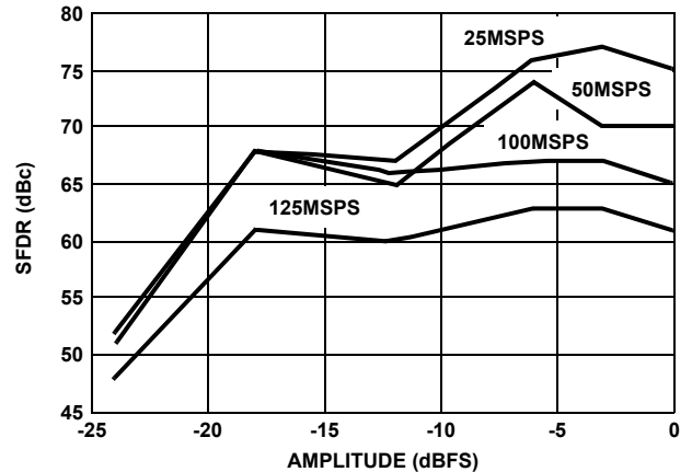
FIGURE 6. SFDR vs AMPLITUDE, f_{CLK}/f_{OUT} = 10
