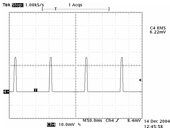
Figure 11. Short Circuit Behavior (typ)
