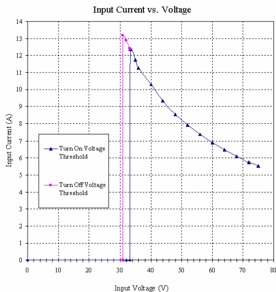
Figure 2. Undervoltage Lockout Characteristics (typ)
